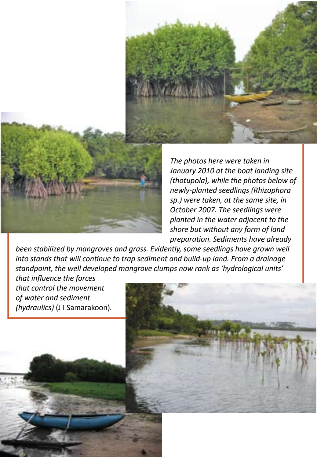
Fig. 3.10 - Rekawa Lagoon, mangrove rehabilitation in the post-tsunami period
